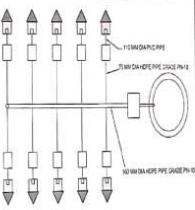
LAYOUT FOR COMMUNITY LEACH PIT WITH SILT CHAMBERS FOR 10 HOUSEHOLD
