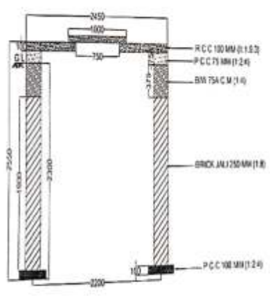
COMMUNITY LEACH PIT WITH SILT FOR 10 HOUSEHOLD ALL DIMENSIONS IN MM
